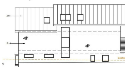
Elevation (South West) / Section BB As Proposed
